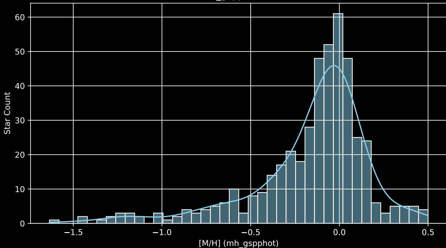
APOGEE DR17 Field: [150+04 [M/H] (mh_gspphot) (n= 456)
