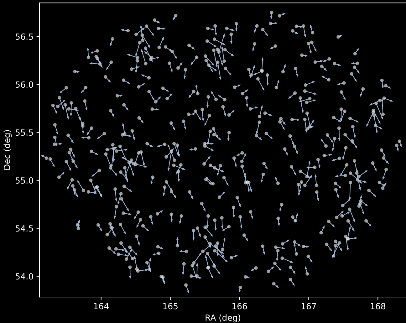
APOGEE DR17 Cluster 1 Proper Motion Vectors (n=393)
