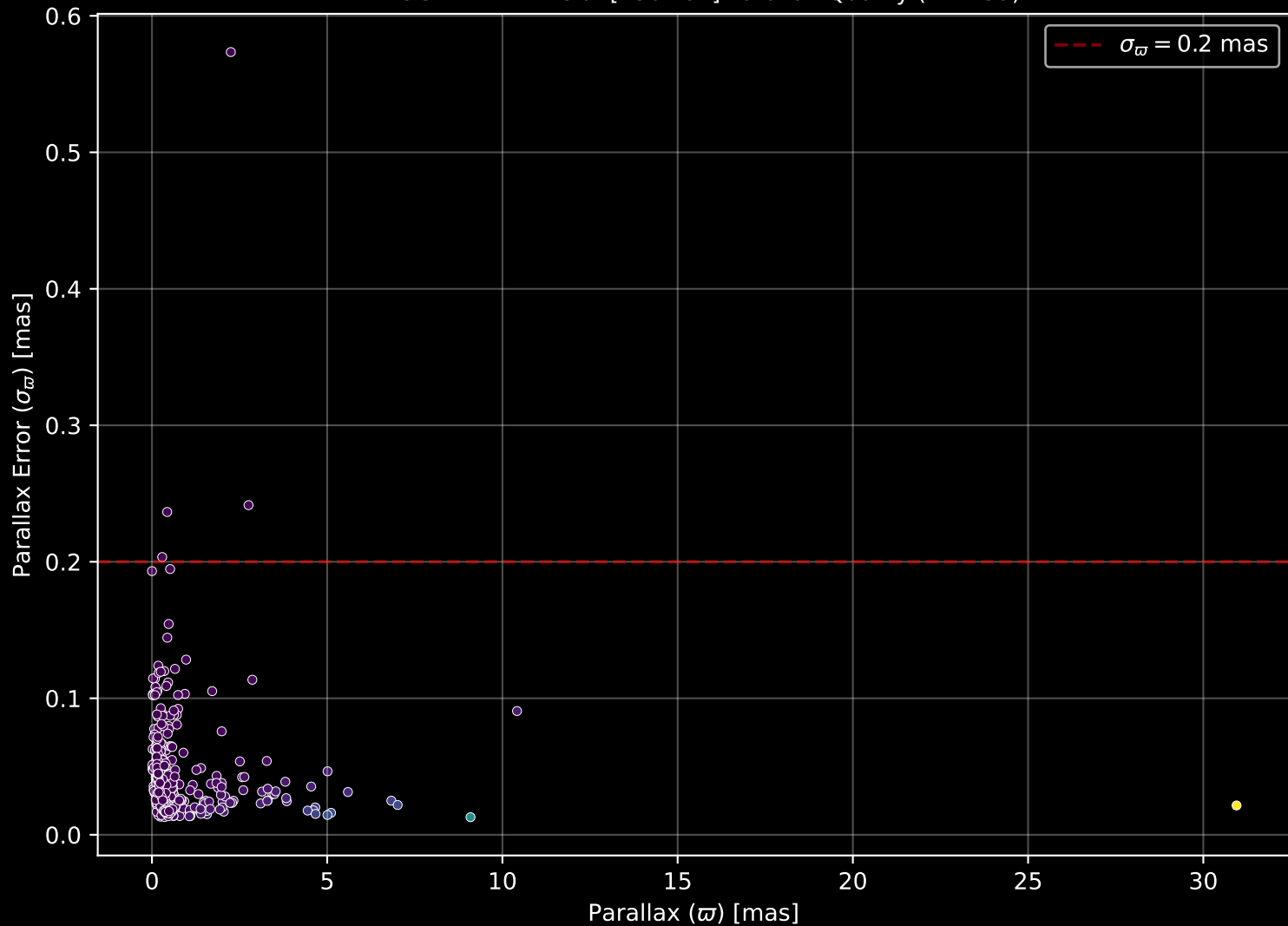
APOGEE DR17 Field: [150+04] Parallax Quality (n= 459)
