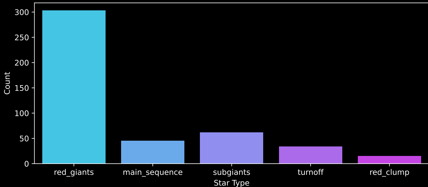
APOGEE DR17 Field: [150+04] Count plot of Star Type
