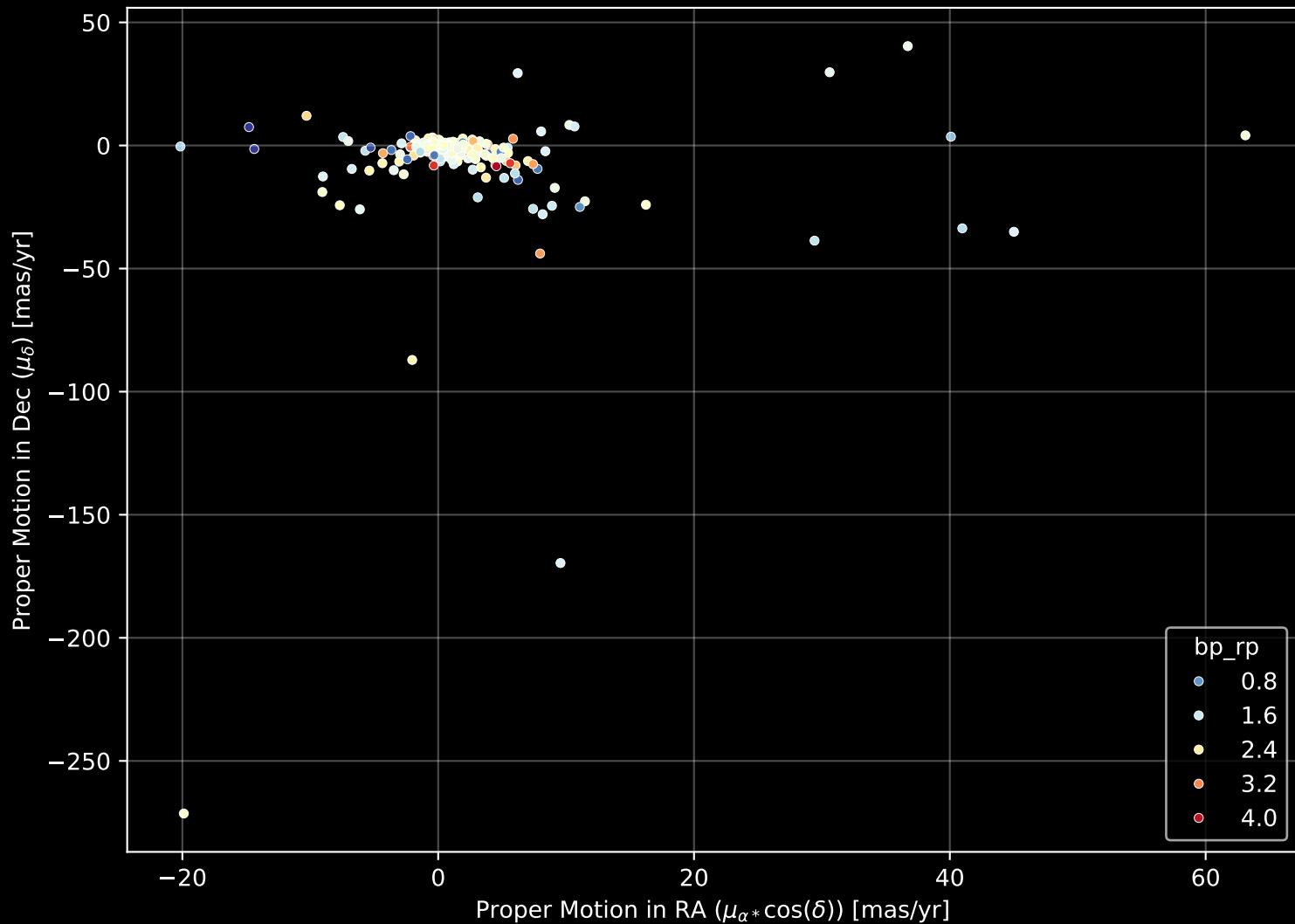
APOGEE DR17 Field: [150+04] Proper Motion Diagram (n= 459)
