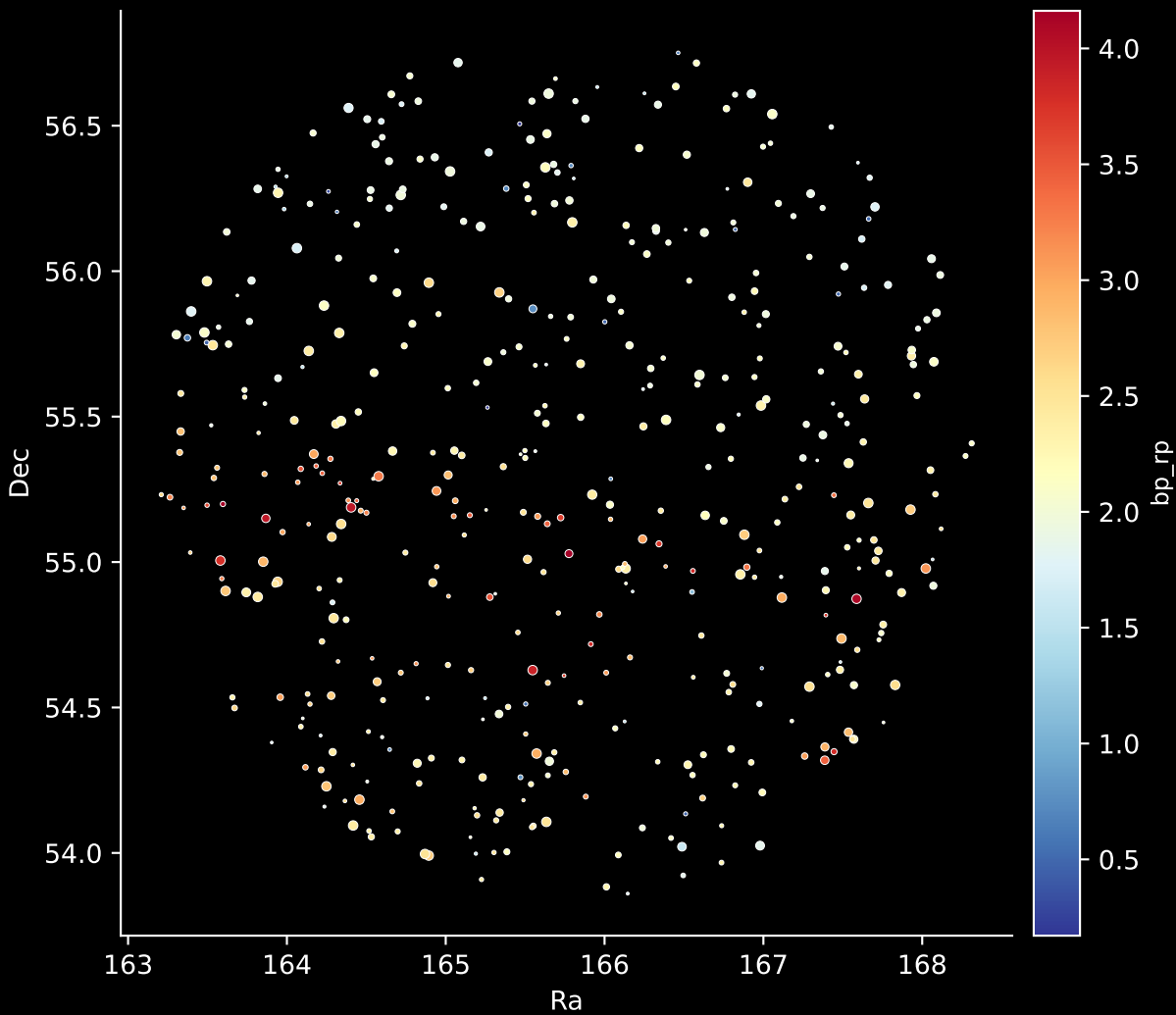
APOGEE DR17 Field: [150+04] Stars: 459
