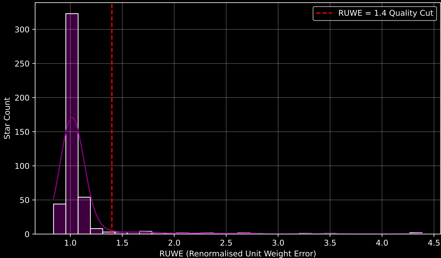
GAPOGEE DR17 Field [150+04] RUWE Distribution (n= 458)
